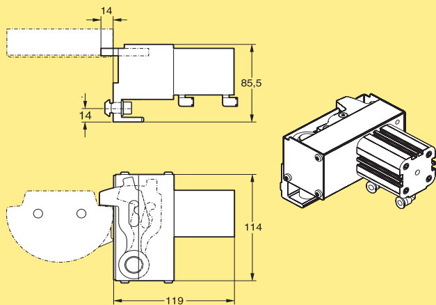
Pneumatic stop device Double-actuated
