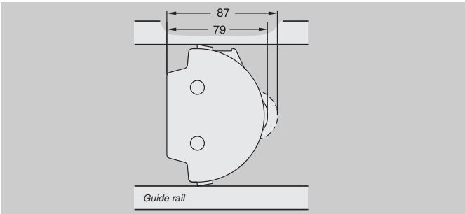
Shock absorber Polyurethane 3926430
