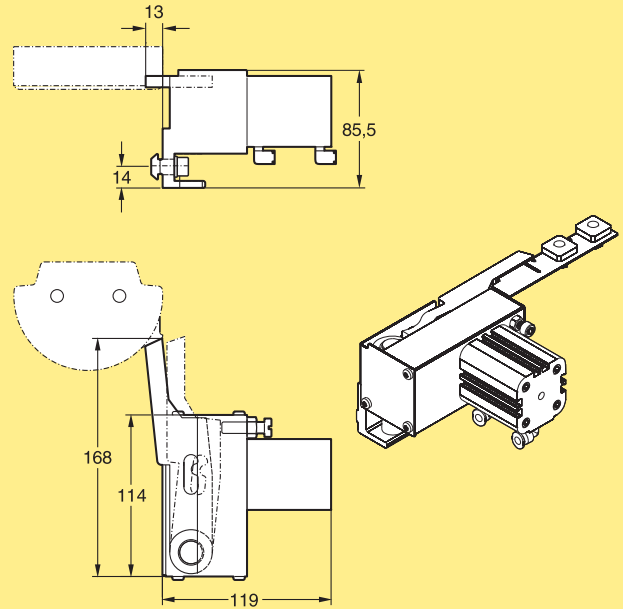
Pneumatic stop for pallet locating station, double-actuated XKPD 32x15 LB
