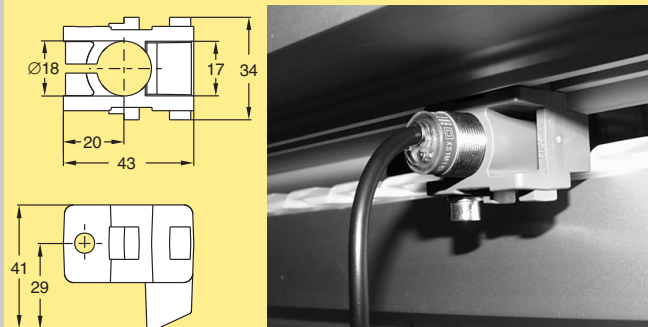
Bracket for horizontal proximity switch Ø18 mm XKPB 18 H Acetal resin. Including screw, T-slot nut and washer
