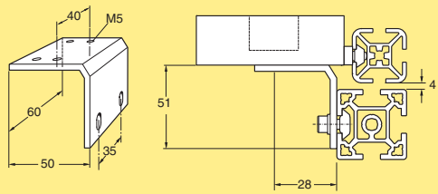
Safety switch bracket kit Aluminium, anodized XFEL 60 WA Including the necessary mounting hardware. For safety switches Schmersal AZ 15/16-B1 and Guardmaster Trojan 5 (not included).
