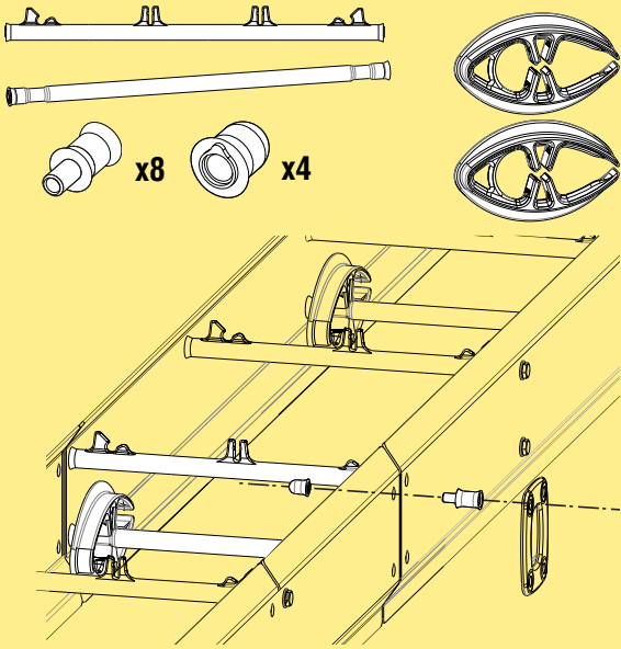
Beam spacer kit
