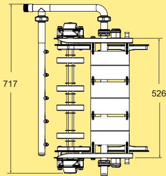
CIP washing unit for plain belt WLNWX A526 CIP
