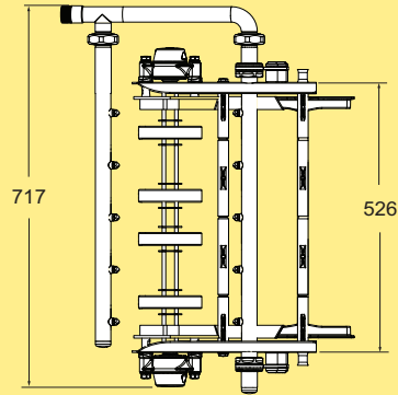
CIP washing unit for flat top belt WLNWX B526 CIP
