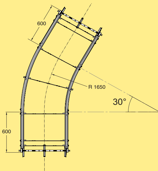
Plain bend, 30°±1° R=1650±10 mm
