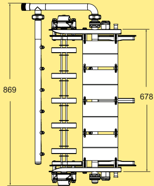
CIP washing unit for plain belt WLNWX A678 CIP
