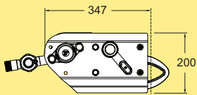
CIP washing unit, WL678X, plain belt
