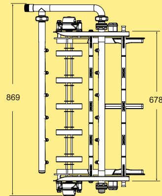
CIP washing unit for flat top belt WLNWX B678 CIP
