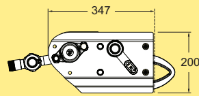
CIP washing unit, WL678X, flat top belt
