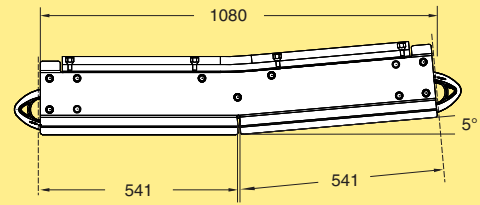
Vertical bend 5°, pos WLBVX 5A222P
