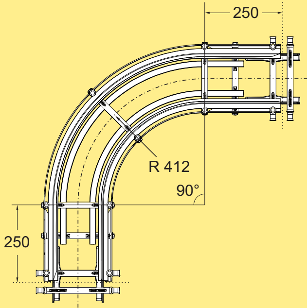
Plain bend, 90°±1° R=412±10 mm WLBPX 90A222
