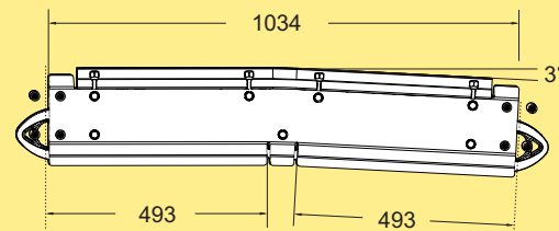
Vertical bend 3°, neg WLBVX 3A222N
