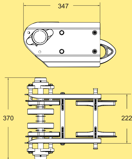
Idler end unit
