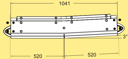
Vertical bend 3°, pos WLBVX 3A222P
