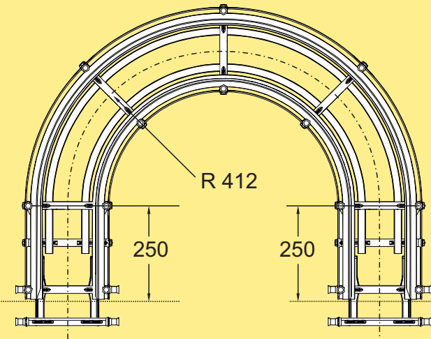
Plain bend, 180°±1° R=412±10 mm WLBPX 180A222
