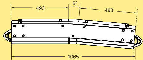
Vertical bend 5°, neg WLBVX 5A222N
