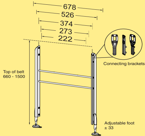
Support module type H WLUFX S01
