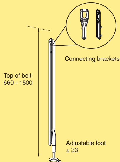
Support module, single leg WLUFX S04
