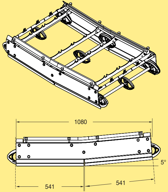
Vertical bend 5°, pos WLBVX 5A678P
