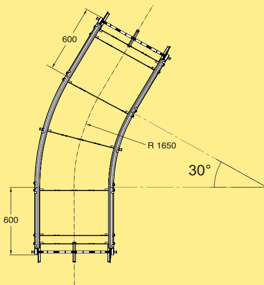
Plain bend, 30°±1°
