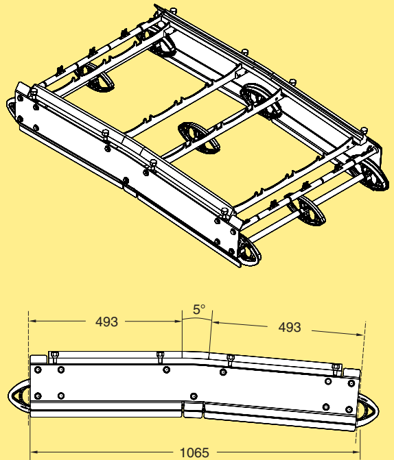
Vertical bend 5°, neg WLBVX 5A678N
