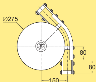
Wheel bend, 45° XLBHX 45R150 Effective track length: 0,30 m (2-way 0,60 m)
