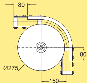
Wheel bend, 90° XLBHX 90R150 Effective track length: 0,40 m (2-way 0,80 m)
