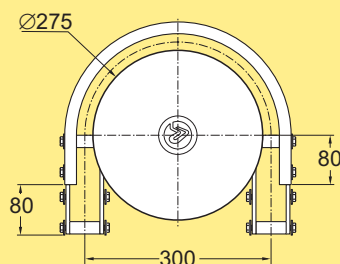
Wheel bend, 180° XLBHX 180R150 Effective track length: 0,65 m (2-way 1,30 m)
