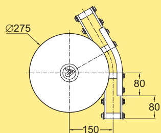
Wheel bend, 30° XLBHX 30R150 Effective track length: 0,25 m (2-way 0,50 m)
