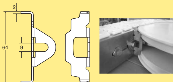
Safety cover for wheel bend XLBHX 5056997 Each item consists of two (2) covers 5056925. Use the existing screw and washer for assembly.
