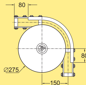
Wheel bend, 90° XLBHX 90R150 Effective track length: 0,40 m (2-way 0,80 m)
