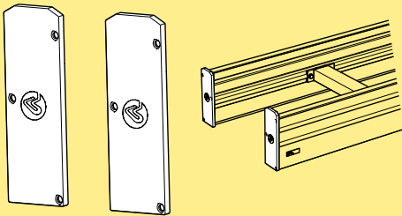
End stop FLX1015275 Used for safety at the end of the module. Including fasteners. Contains 2 pcs.
