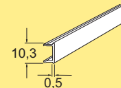
Cover strip for T-slot Length 3 m PVC, grey XCAC 3 P
