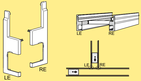
End cap Left side Right side PA, dark grey XCBE 64x189 LE XCBE 64x189 RE
