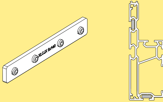
Connecting strip Stainless steel, XLCJX 5x140 Including M8 set screws. Contains 10 pcs
