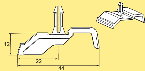
Holder for M12-T splitter cable in cable duct POM, grey FLX1012938
