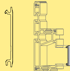
Cover for cable duct, 55 mm. Length 4 m PE, grey XCCC 4x55
